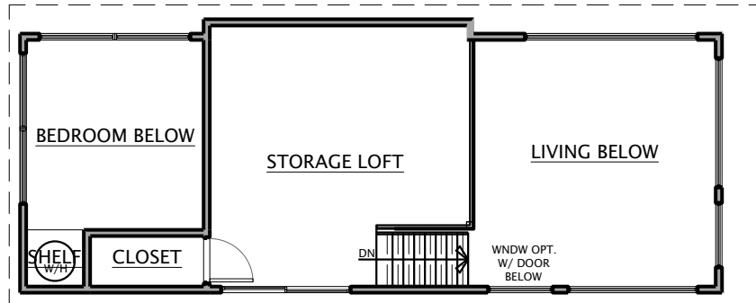
UPPER LOFT - FLOOR PLAN
