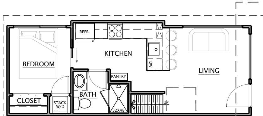
MAIN FLOOR PLAN
