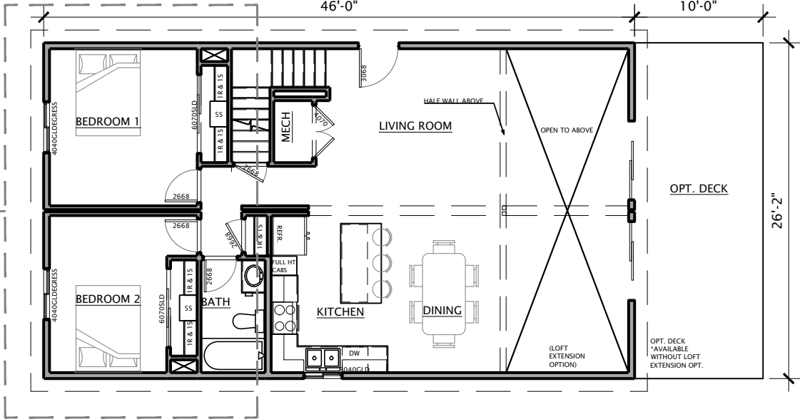
MAIN LEVEL - EXTENDED MODEL W/LOFT OR BONUS 1204 sq. ft.
