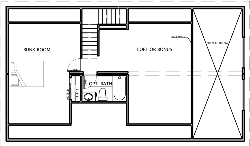
UPPER LEVEL - EXTENDED MODEL W/LOFT OR BONUS 677 sq. ft.
