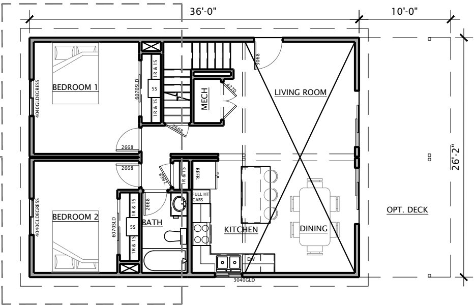
MAIN LEVEL 942 sq ft
