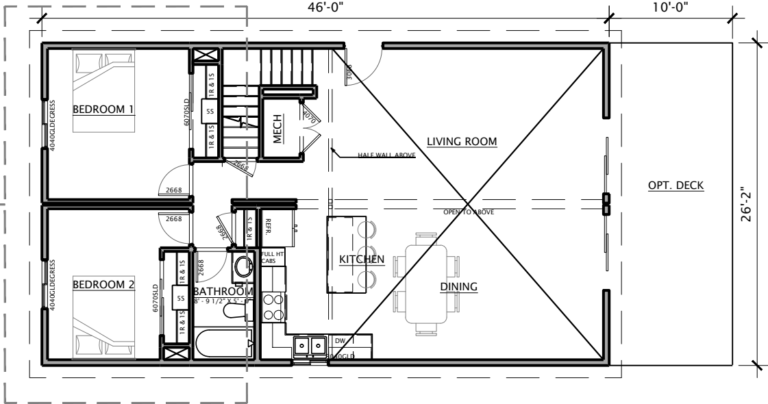
MAIN LEVEL - EXTENDED MODEL 1204 SQ. FT.
