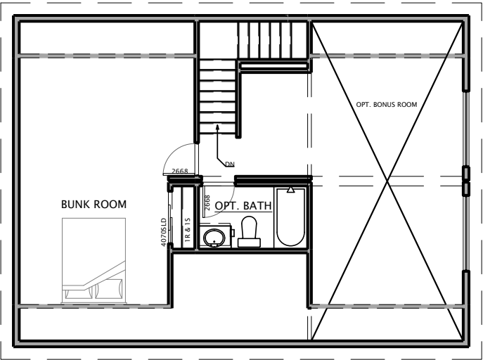
UPPER LEVEL 425 sq. ft. UPPER LEVEL WITH BONUS ROOM 677 SQ. FT.
