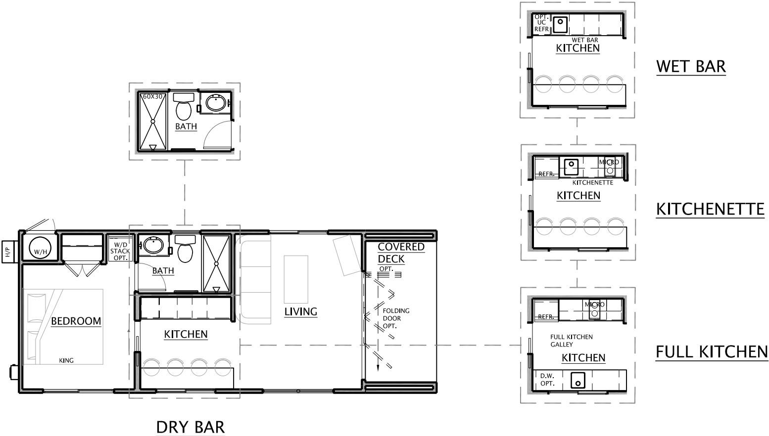
MYSA 400 - FLOOR PLAN © IRONTOWN HOMES
