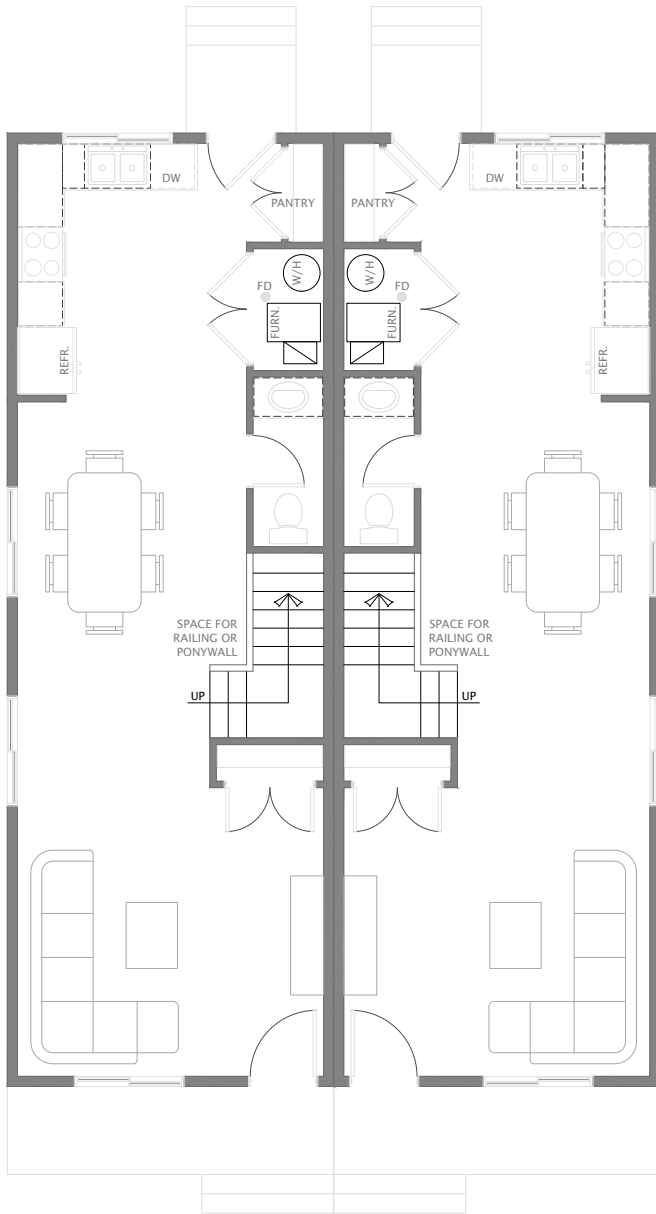
BERKELEY DUPLEX, 2 BED - FLOOR PLAN © IRONTOWN MODULAR
