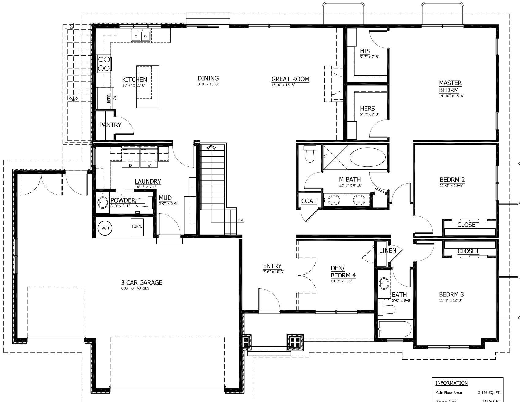
ASHLEE RIDGE 2146 - FLOOR PLAN © IRONTOWN HOMES
