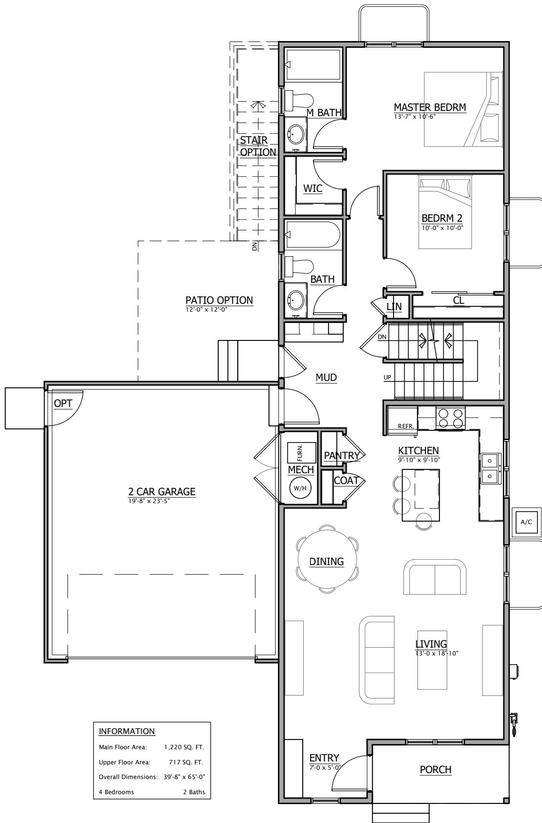
EAGLE LANDING 1976 - 4 BEDROOM STANDARD MAIN FLOOR PLAN © IRONTOWN HOMES
